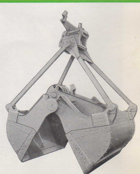
Fig. 26. Blaw-Knox two-line lever arm type wide rehandling type bucket. Size No. 7600 with stiffbacks and corner reinforcements.
