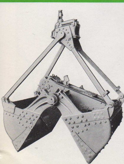
Fig. 24. Blaw-Knox two-line lever arm type wide rehandling bucket. Size No. 7150.
